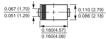
DO-214AC
