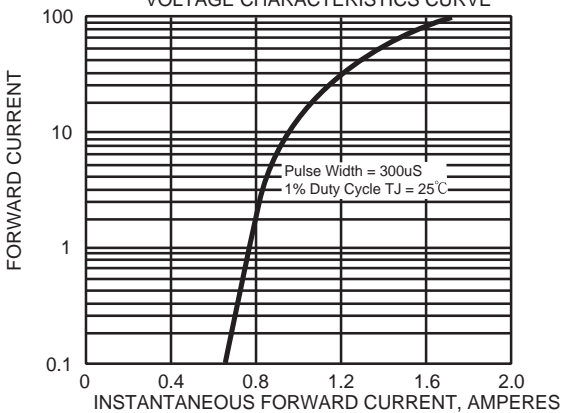
FIG. 11 - INSTANTANEOUS FORWARD VOLTAGE CHARACTERISTICS CURVE
